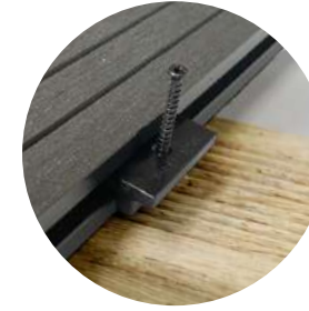
CLIP & SCREW
